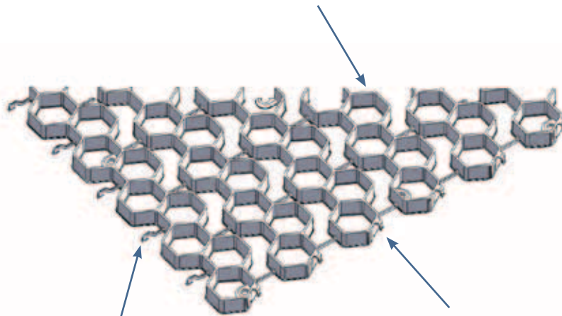
Side-to-side clips make connections between rolls.
